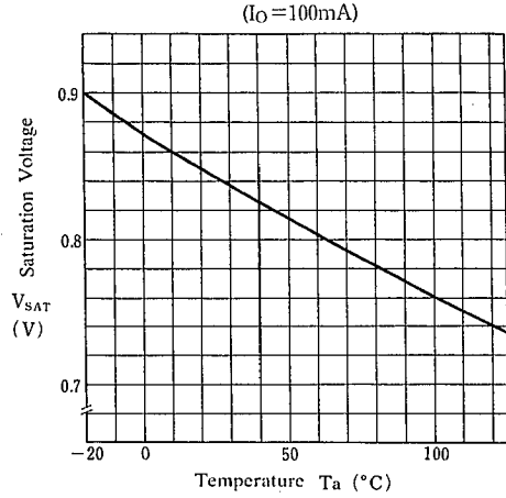
< Output Section > Saturation Voltage vs. Temperature ( I_o=100\text{mA} )
