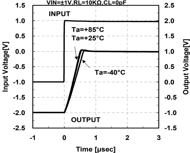
Pulse Response (Rise)
