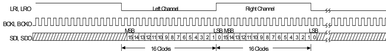
Fig. 4-13 I²S Data Format 32Fs, 16bit Data
