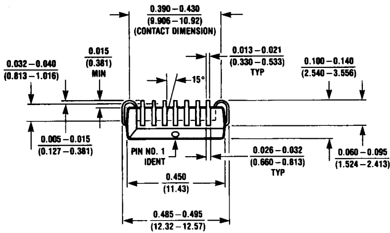
32-Lead PLCC Package Order Number NMC27C256
