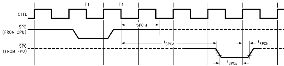
TL/EE/9424-39 FIGURE 4-12. SPC Timing After transferring the last operand to the FPU, the CPU turns OFF the output driver and holds SPC high with an internal 5 k \Omega pullup.
