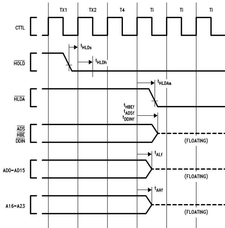
FIGURE 4-7. \overline{HOLD} Acknowledge Timing (Bus Initially Not Idle)
