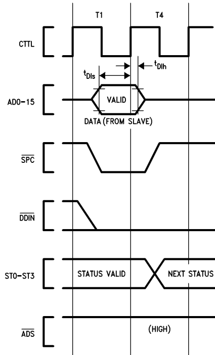
TL/EE/9424-38 FIGURE 4-11. Slave Processor Read Timing
