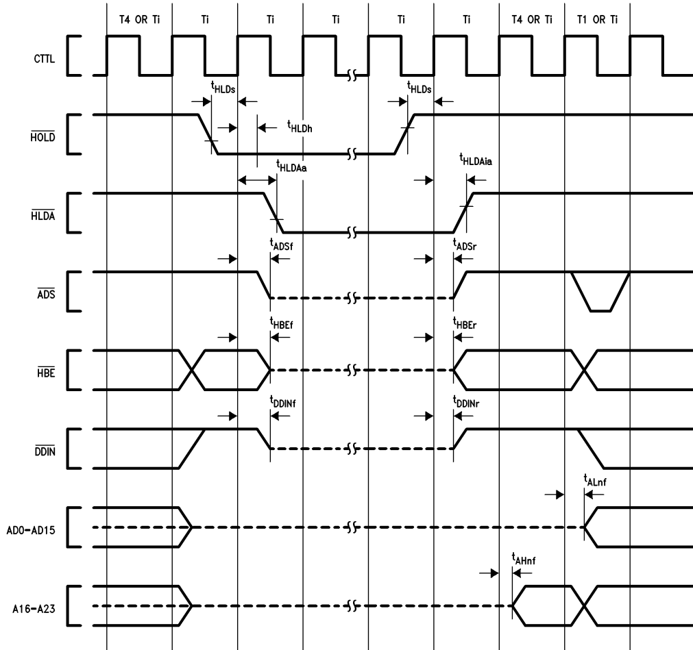
FIGURE 4-8. \overline{\text{HOLD}} Timing (Bus Initially Idle)
