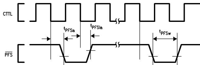
TL/EE/9424-40 FIGURE 4-13. PFS Signal Timing
