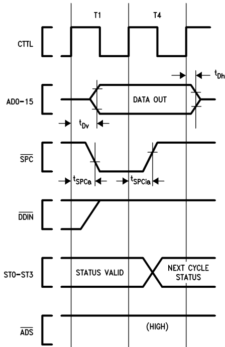
TL/EE/9424-37 FIGURE 4-10. Slave Processor Write Timing
