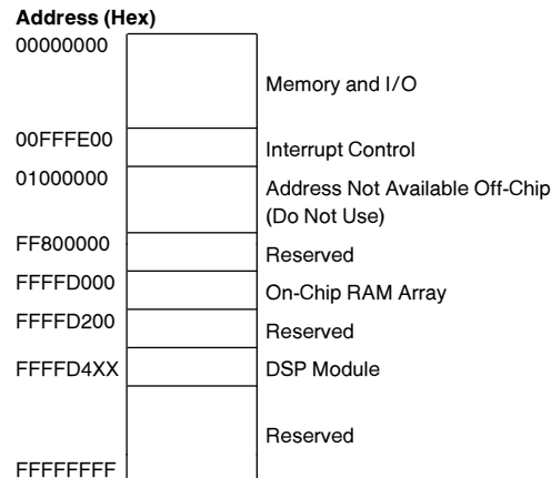
FIGURE 2-9. NS32FX16 Address Mapping
