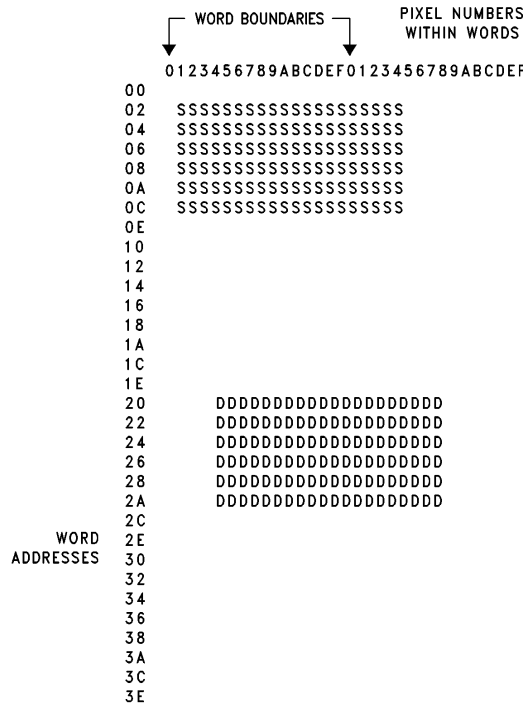
FIGURE 2-15. 32-Pixel by 32-Scan Line Frame Buffer
