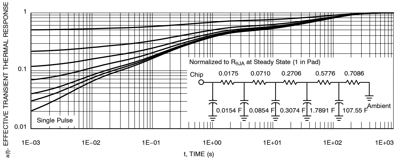
Figure 13. Thermal Response
