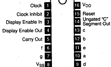
NTE4026B 16-Lead DIP, See Diag. 249 Decade Counter/Divider w/Decoded Seven-Segment Display Outputs & Display Enable
