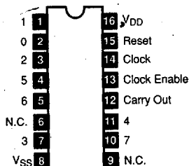
NTE4022B 16-Lead DIP, See Diag. 249 Octal Counter/Divider w/8 Decoded Outputs
