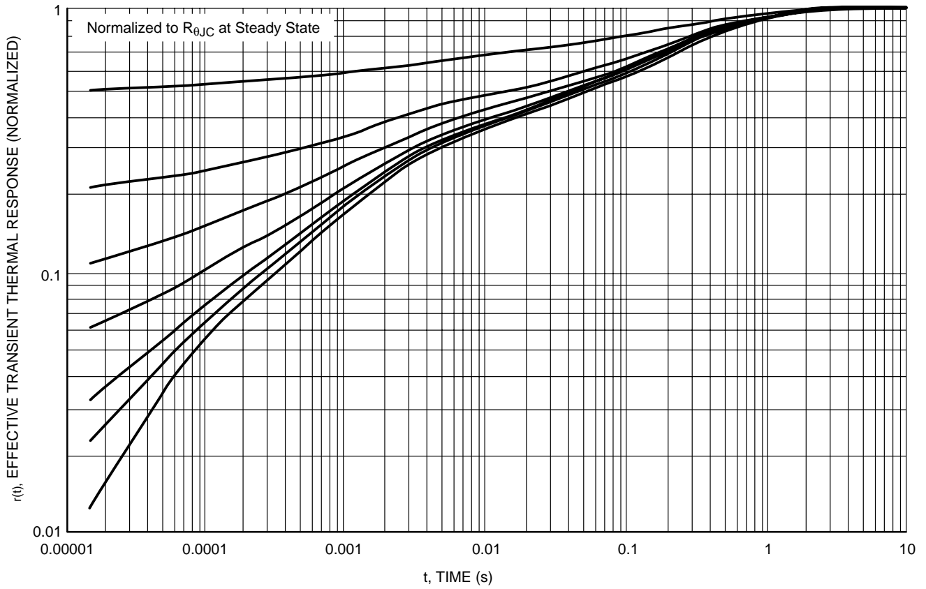
Figure 12. Thermal Response
