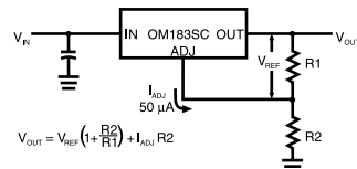
Basic Adjustable Regulator
