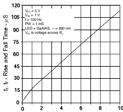
Typical Rise and Fall Time vs. Load Resistance
