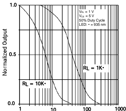
Normalized Output vs. Frequency
