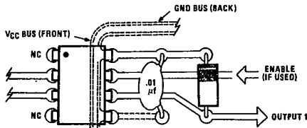
Figure 9. Recommended Printed Circuit Board Layout
