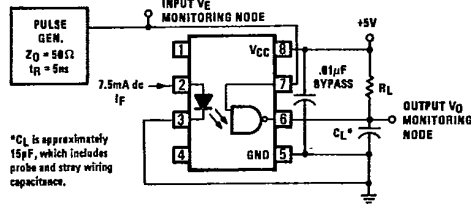
Figure 10. Test Circuit for T_{ELH} and T_{EHL}
