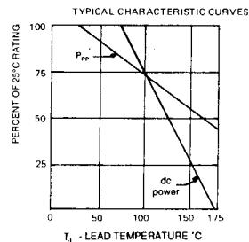
FIGURE 1 POWER DERATING CURVE
