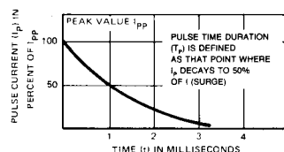
FIGURE 2 PULSE WAVEFORM FOR EXPONENTIAL SURGE
