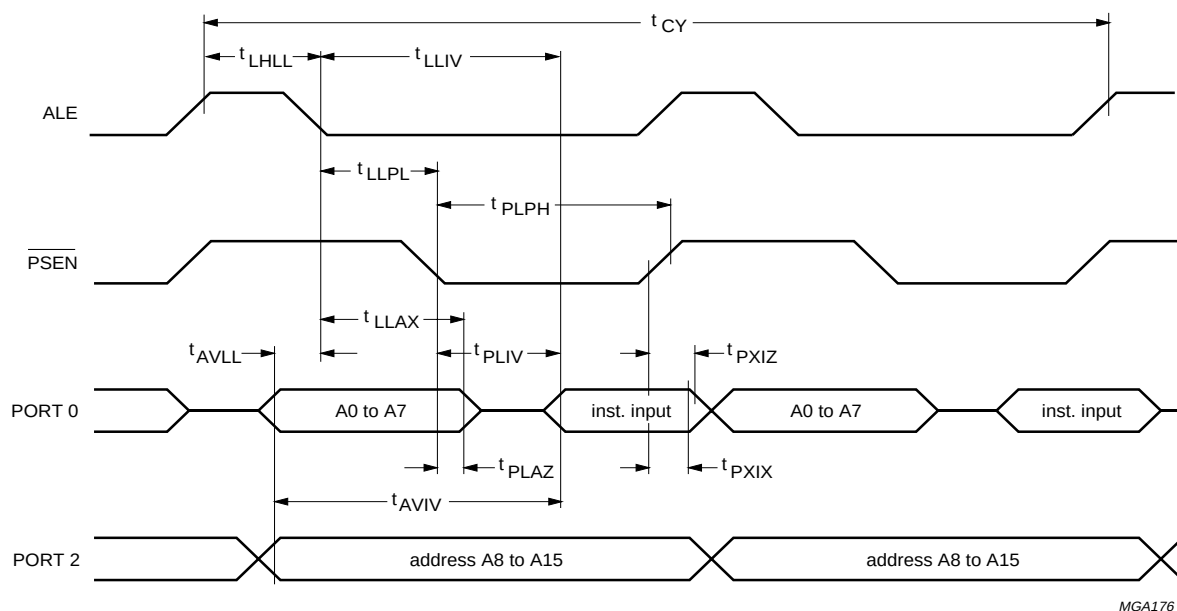
Fig.22 Read from program memory.
