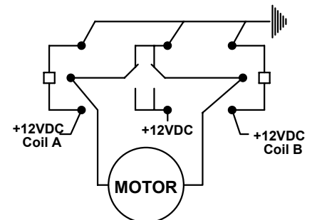
Typical Schematic Motor on, off, Fwd. & Rev.
