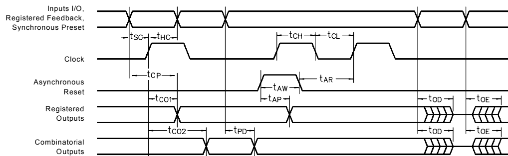
Figure 7 - Switching Waveforms
