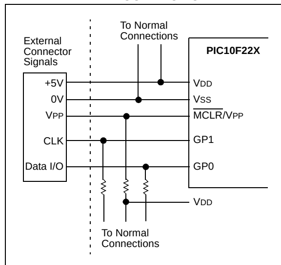
FIGURE 8-10: TYPICAL IN-CIRCUIT SERIAL PROGRAMMING CONNECTION
