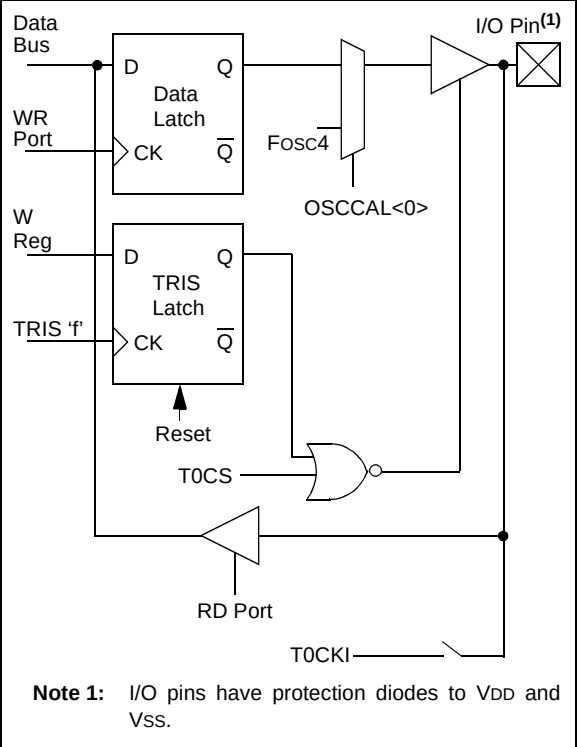
FIGURE 5-3: BLOCK DIAGRAM OF GP2
