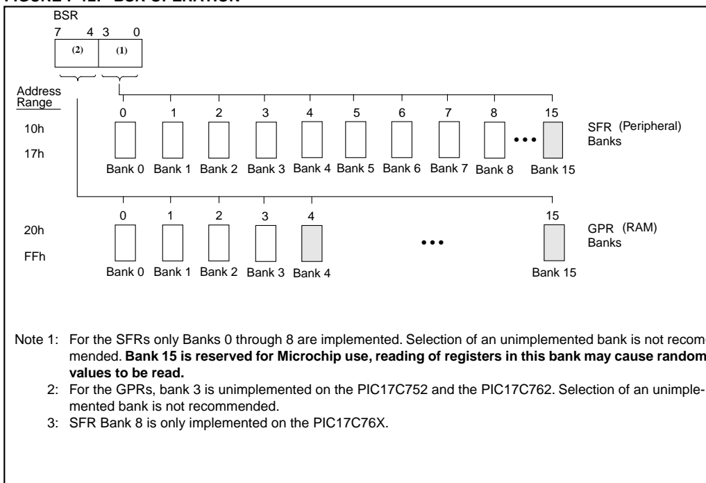
FIGURE 7-12: BSR OPERATION
