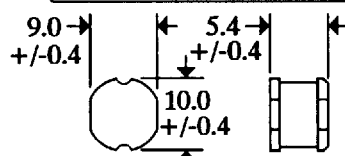
Terminal Dimensions
