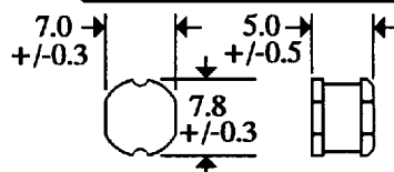
Terminal Dimensions
