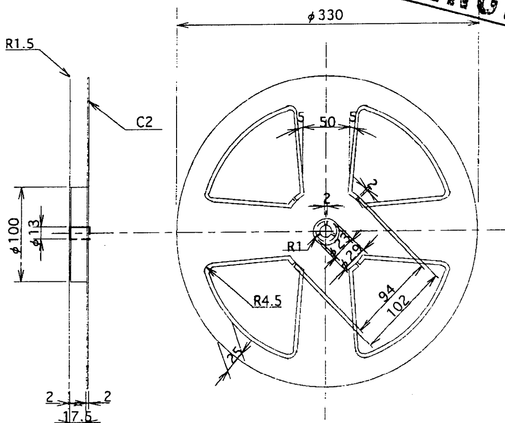
Fig. B Reel structure and Dimensions
