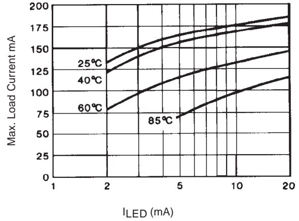
Figure 2. Typical Control Current Requirements
