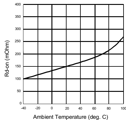
Figure 4. Typical On-Resistance
