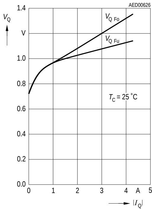
Diode Forward Voltage versus Output Current
