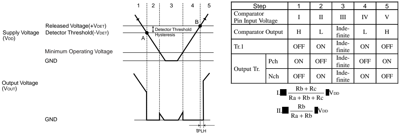
Figure 2. Operation Diagram
