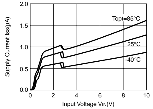
R3111x271C
