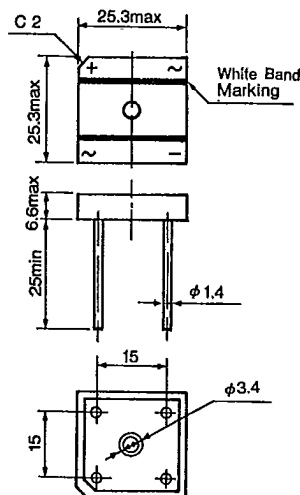
Outline Drawing ⑤3
