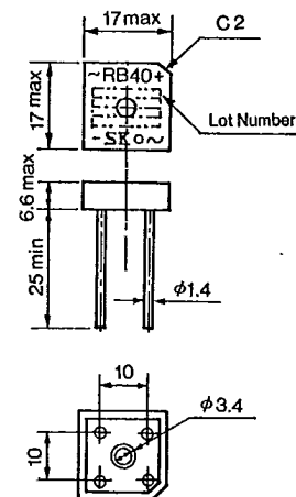
Outline Drawing ⑤2
