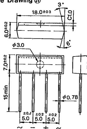
Outline Drawing ⑤1
