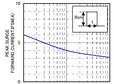
IFSM-t CHARACTERISTICS
