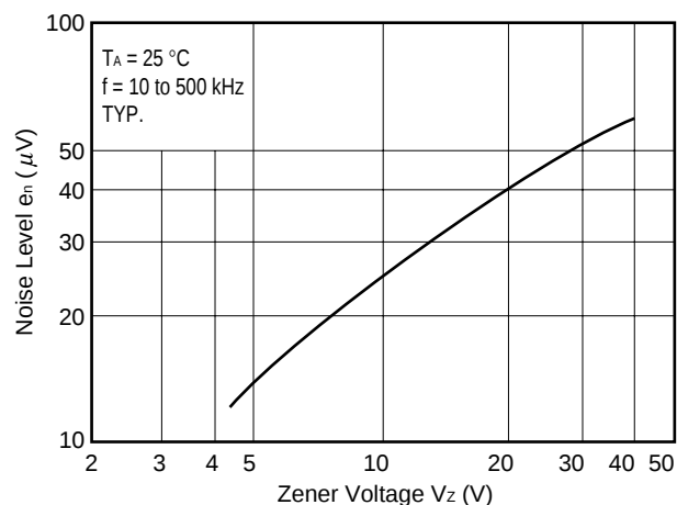
Fig. 8 e_n -V z CHARACTERISTICS
