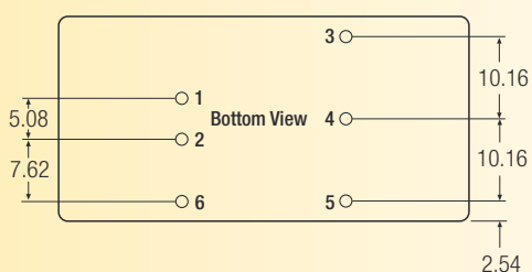
REC10-S_DRW(Z)/H/CTRL
