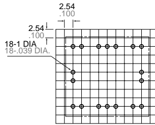
PC board pattern (Copper-side view)
