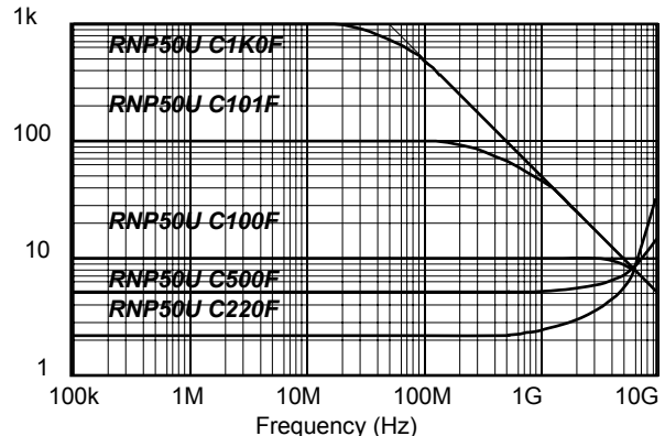
Impedance (ohm)
