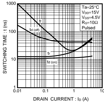
Fig.2 Switching Characteristics
