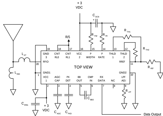
ASH Receiver Application Circuit ASK Configuration
