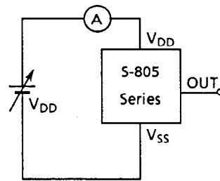
(4) Current consumption
