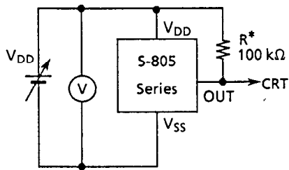
(1) Detection voltage
