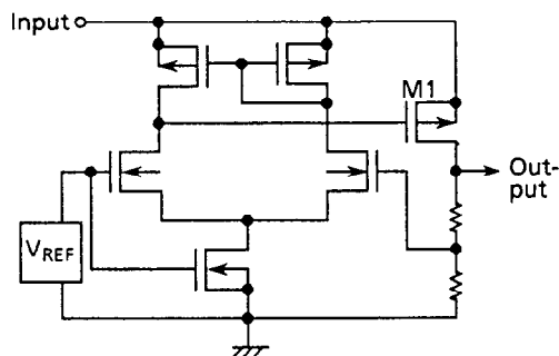
Figure 5 Voltage regulator with built-in MOS FET
