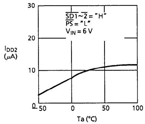
4-4-2 I_{DD2} - Temperature
