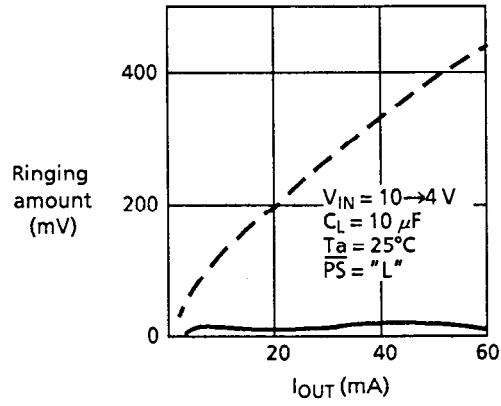
2.2 V_{OUT1}, V_{OUT2}
