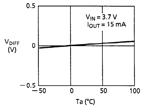
1-2-2 V_{DIFF} -Temperature
