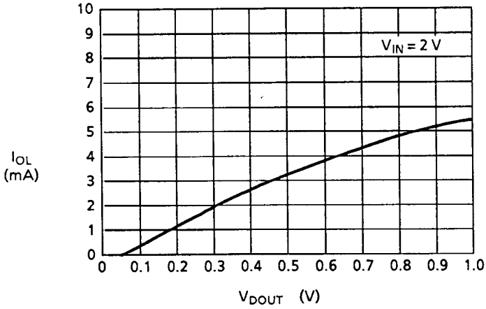
2-2-1 I_{OL} - V_{DOUT}
