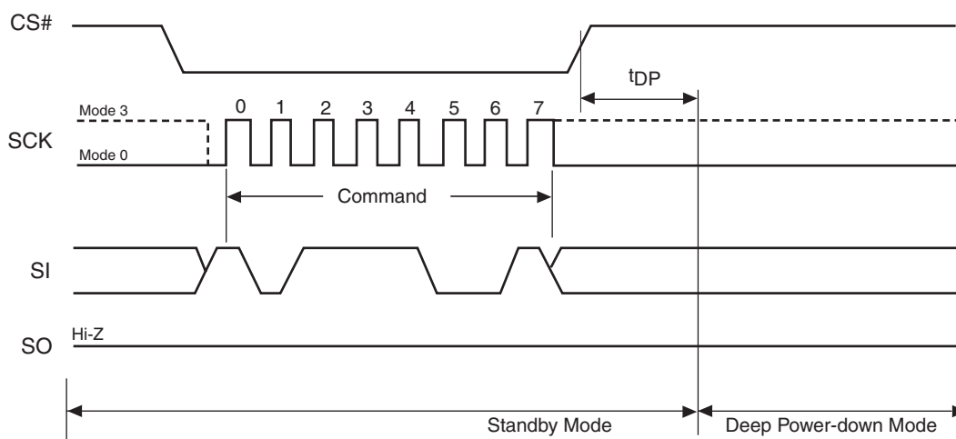
Figure 9.12 Deep Power Down (DP) Command Sequence
