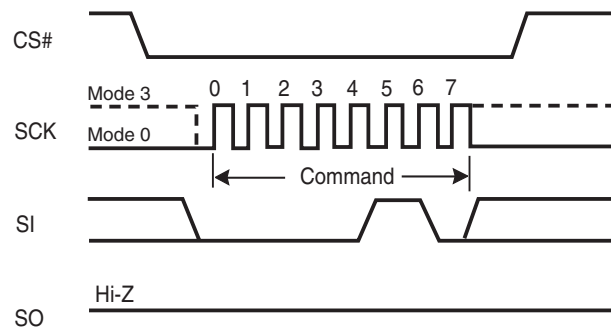
Figure 9.5 Write Enable (WREN) Command Sequence
