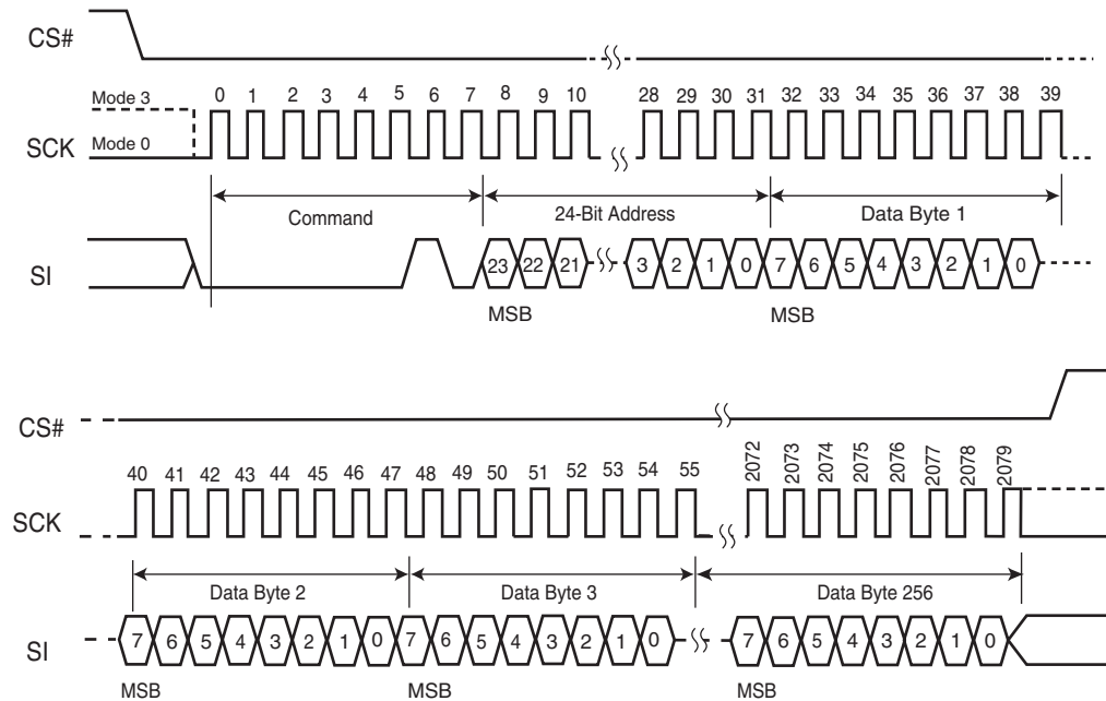
Figure 9.9 Page Program (PP) Command Sequence
