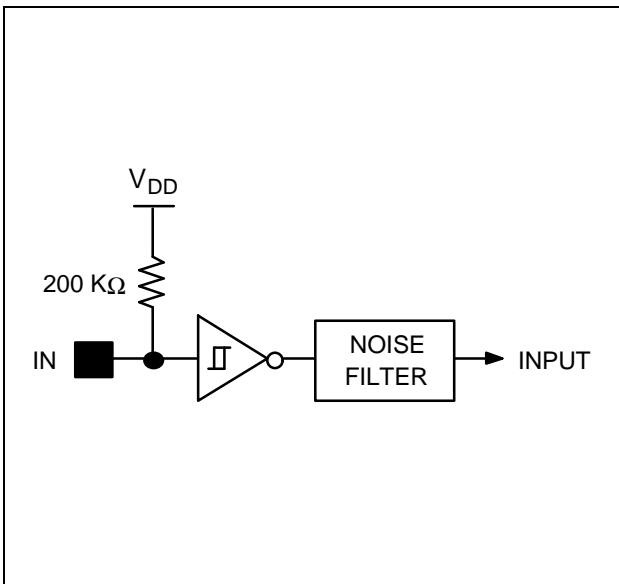
Figure 1-3. Pin Circuit Type 1 (RESET)
