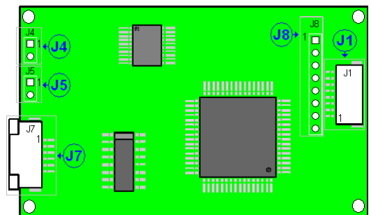
Figure 3. Connector Locations
