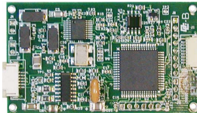
Figure 1. S4100 Multi-Function Reader Module
