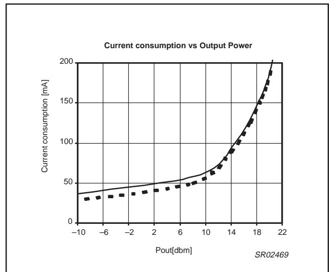
Figure 8. Current consumption vs. output power
