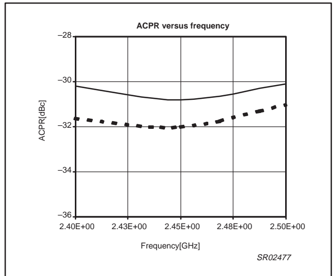
Figure 16. ACPR vs. frequency
