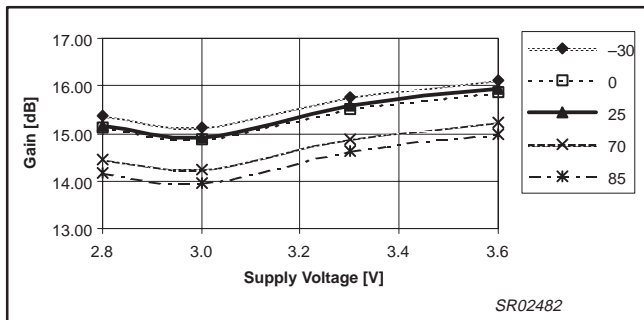
Figure 21. Gain vs. supply voltage, mode = high
