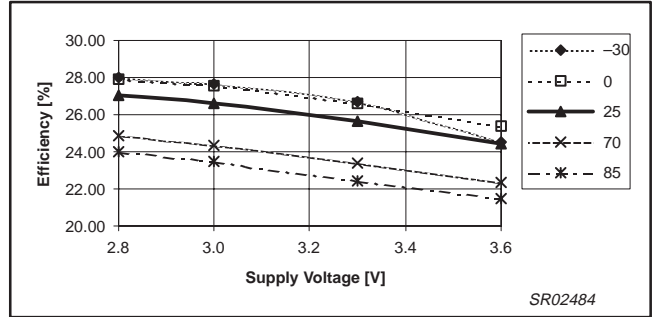
Figure 23. Efficiency vs. supply voltage, mode = high
