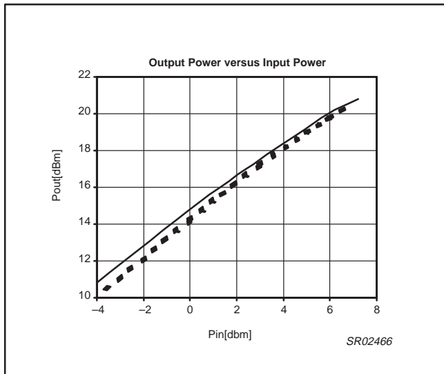
Figure 5. Output power vs. input power
