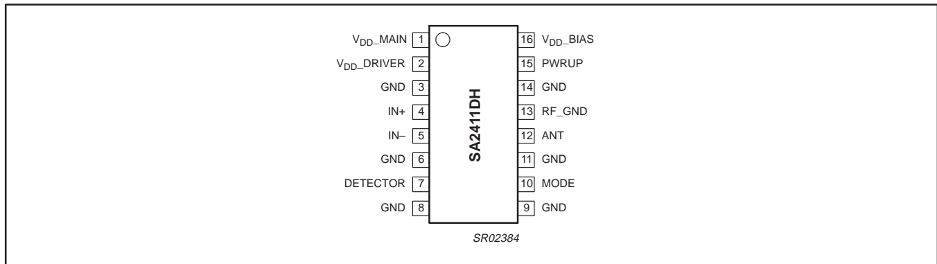
Figure 2. Pin configuration
