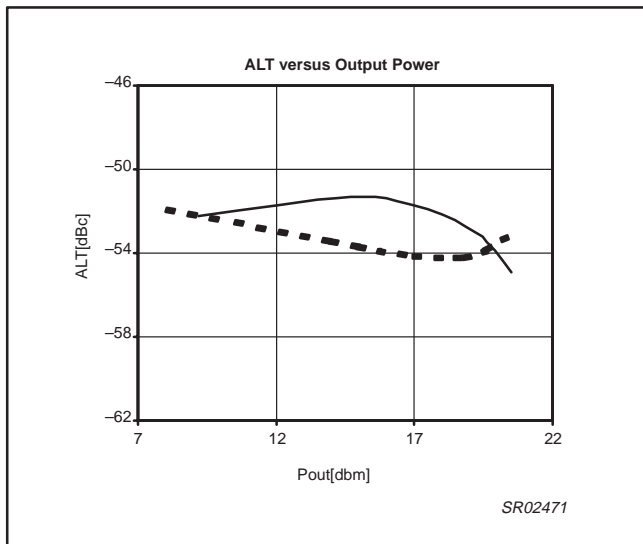
Figure 10. ALT vs. output power
