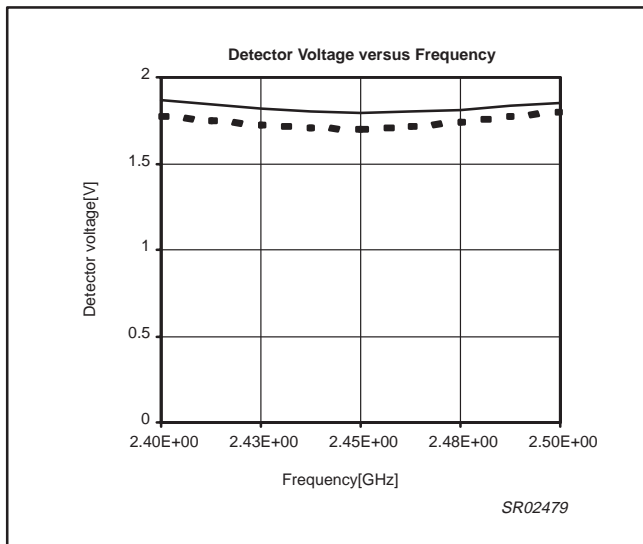
Figure 18. Detector voltage vs. frequency
