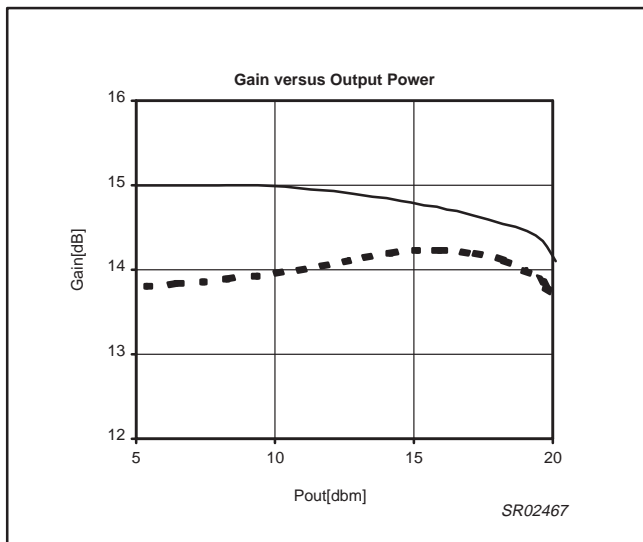
Figure 6. Gain vs. output power
