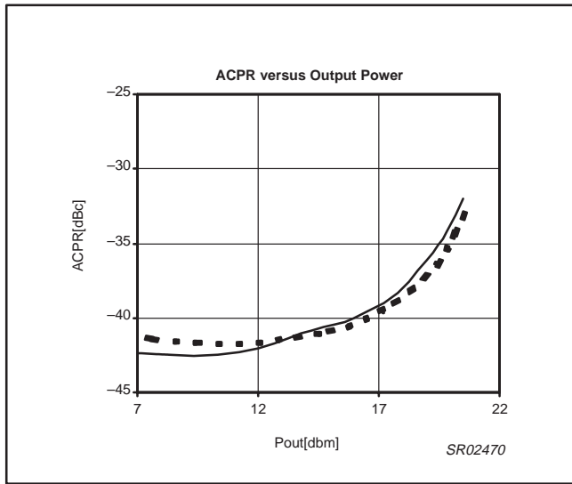
Figure 9. ACPR vs. output power
