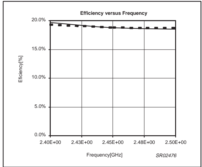
Figure 15. Efficiency vs. frequency
