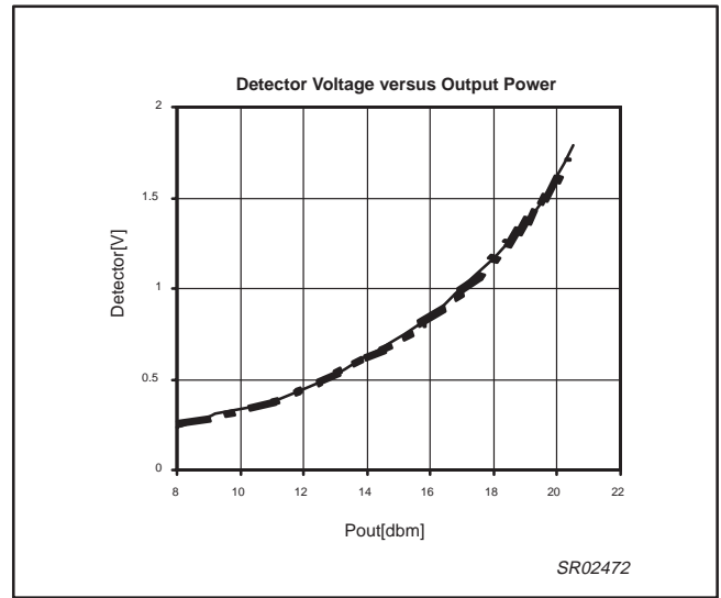
Figure 11. Detector voltage vs. output power
