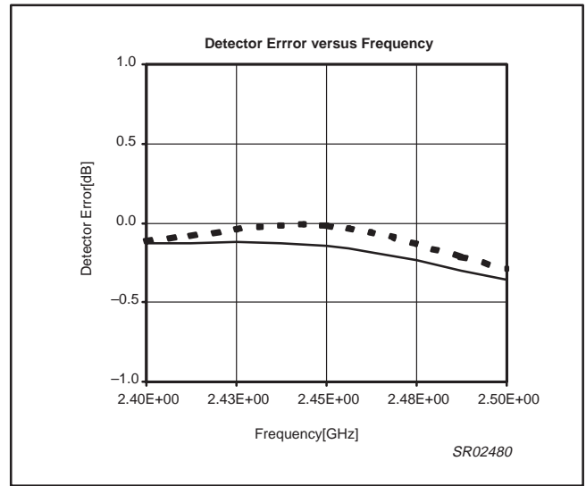
Figure 19. Detector error vs. frequency
