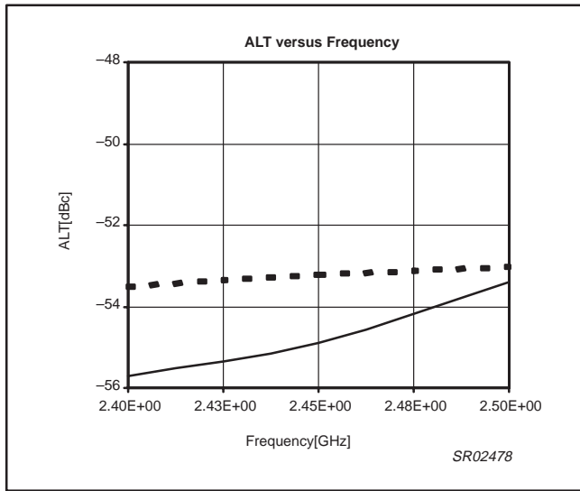
Figure 17. ALT vs. frequency
