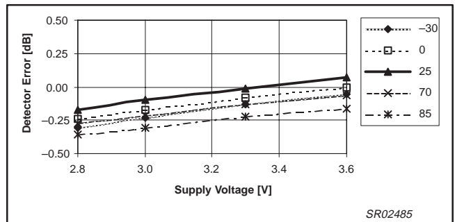
Figure 24. Detector error vs. supply voltage, mode = high
