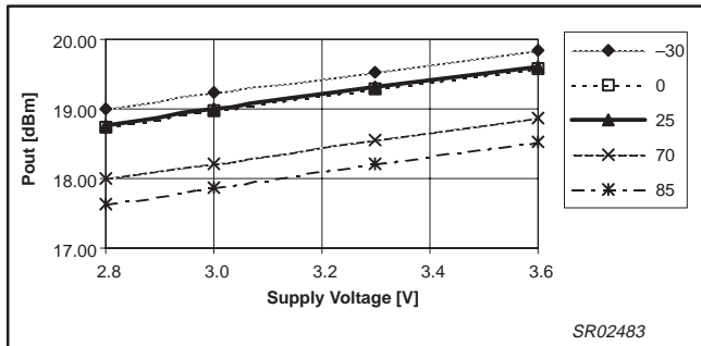
Figure 22. Output power vs. supply voltage, mode = high
