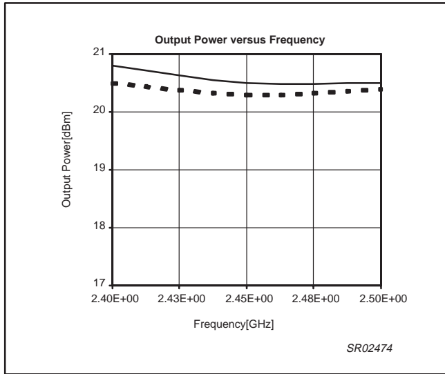
Figure 13. Output power vs. frequency
