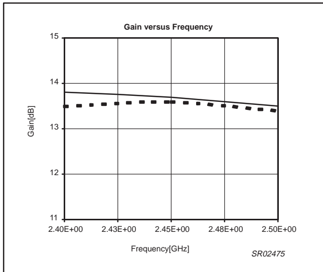
Figure 14. Gain vs. frequency
