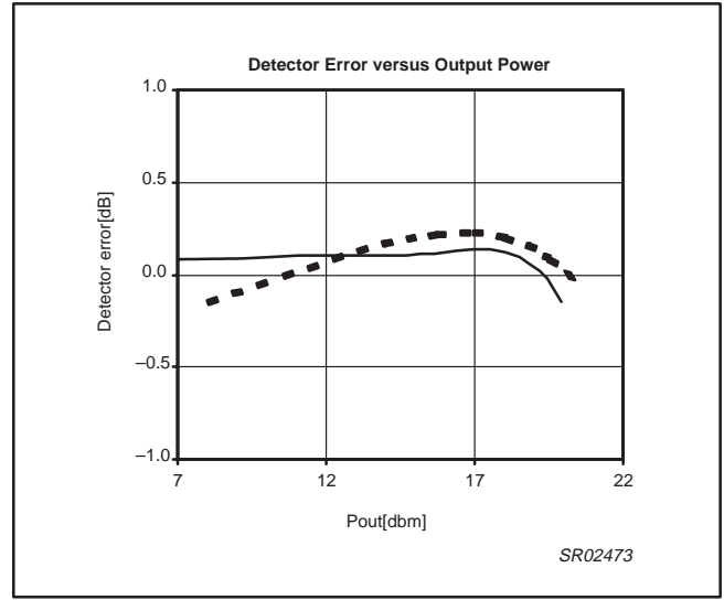
Figure 12. Detector error vs. output power
