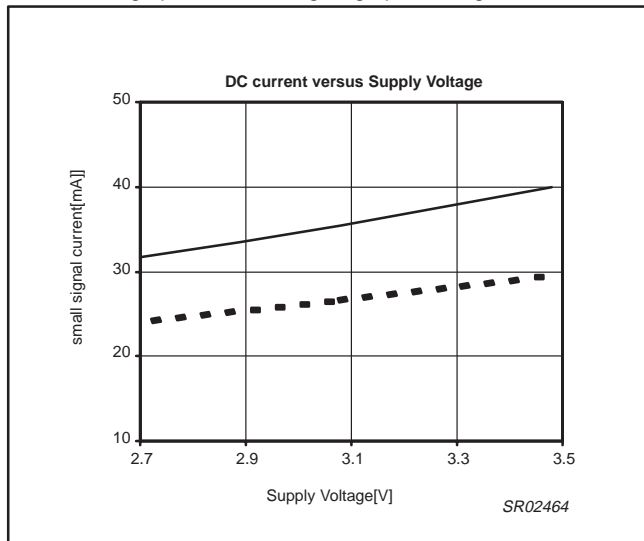
Figure 3. DC current vs. supply voltage
