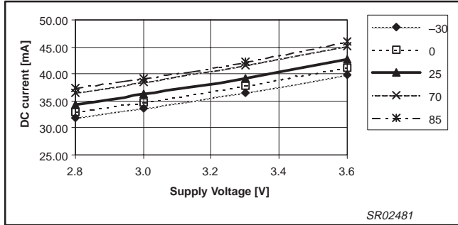
Figure 20. DC current vs. supply voltage, mode = high
