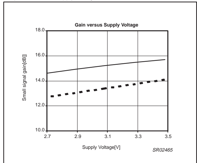
Figure 4. Gain vs. supply voltage
