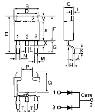
TO-252AA (DPAK)
