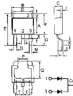
TO-252AA (DPAK)
