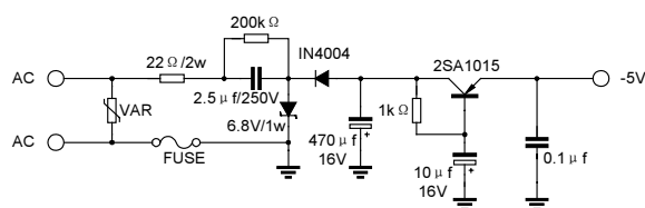
Supply Circuit
