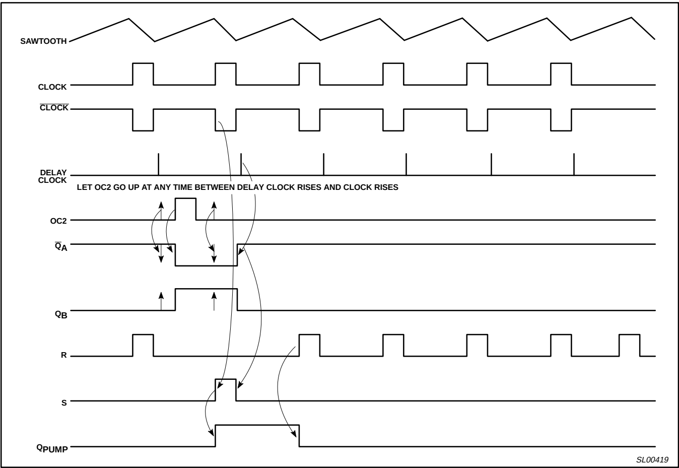
Figure 32. Fault Cycle
