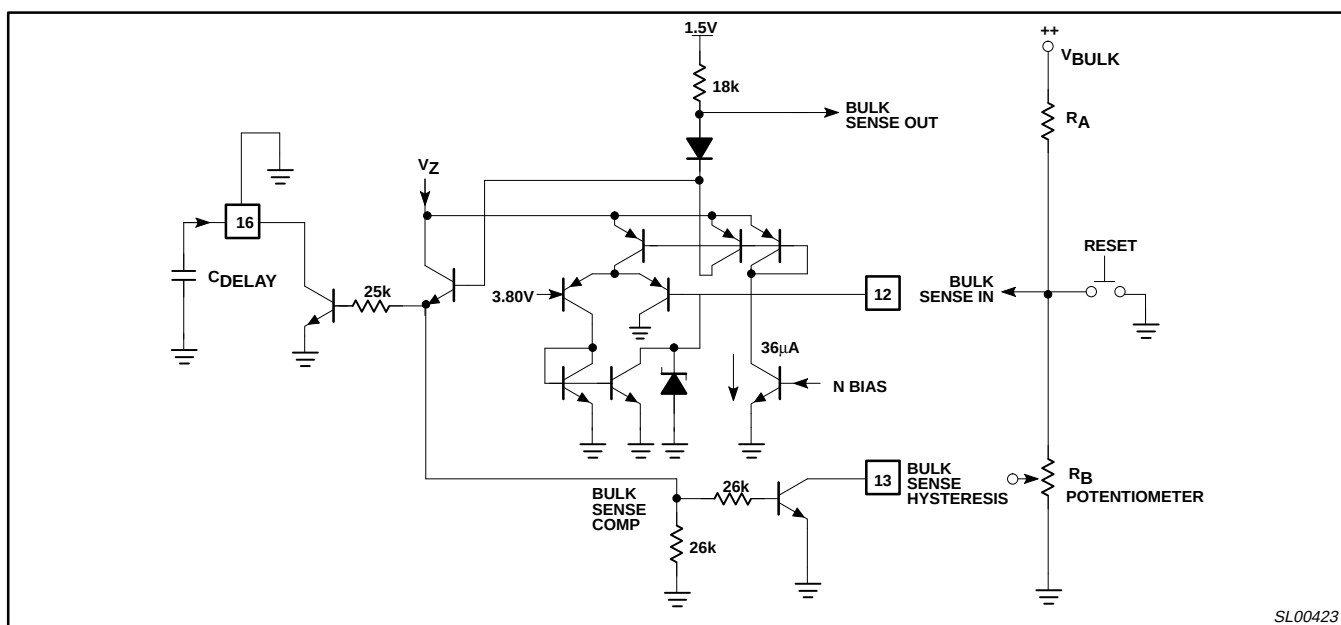
Figure 36. Bulk-Sense Comparator
