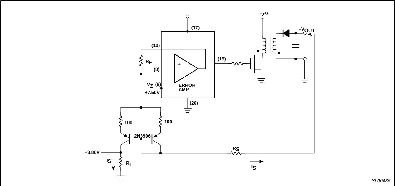
Figure 47. NE5562 Flyback Converter
