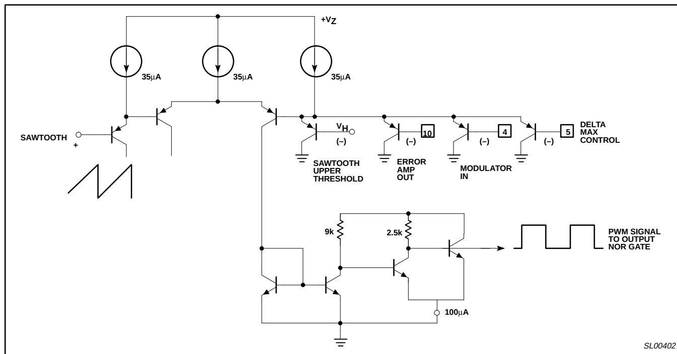
Figure 15. PWM Comparator
