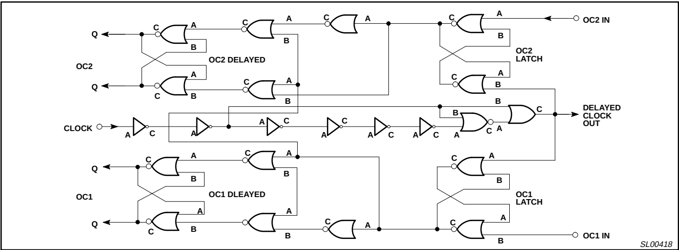
Figure 31. Overcurrent Logic
