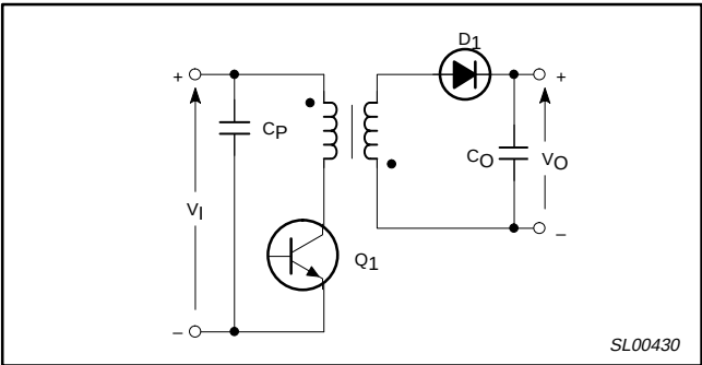
Figure 43. Isolated Secondary
