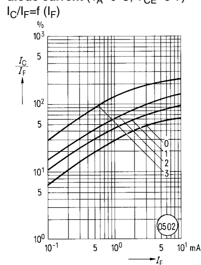
Figure 4. Current transfer ratio versus diode current ( T_A=0\text{ }^\circ\text{C} , V_{CE}=5\text{ V} ) I_C/I_F=f(I_F)
