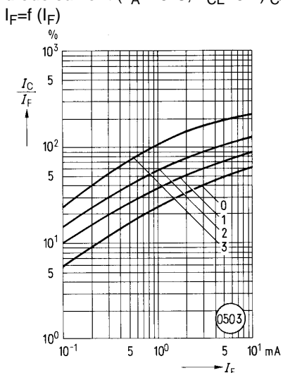
Figure 5. Current transfer ratio versus diode current ( T_A=25\text{ }^\circ\text{C} , V_{CE}=5\text{ V} ) I_C/I_F=f(I_F)
