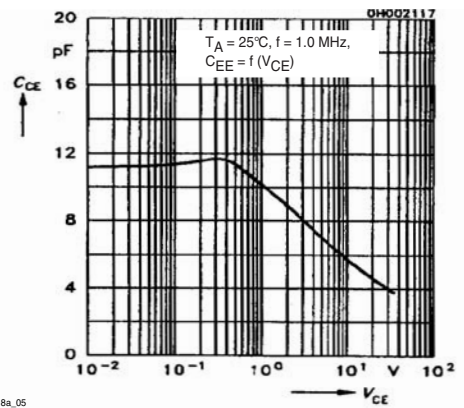
Figure 8. Transistor Capacitance
