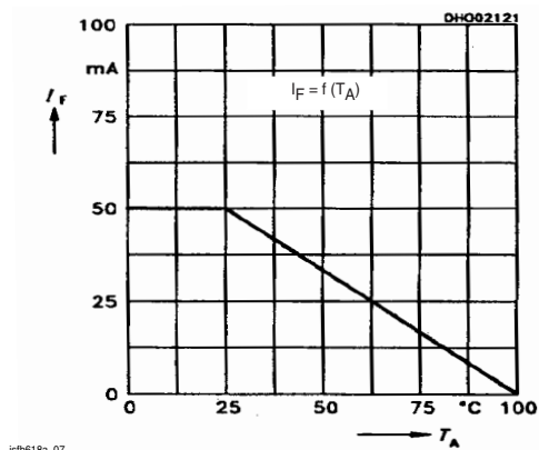
Figure 10. Permissible Forward Current Diode
