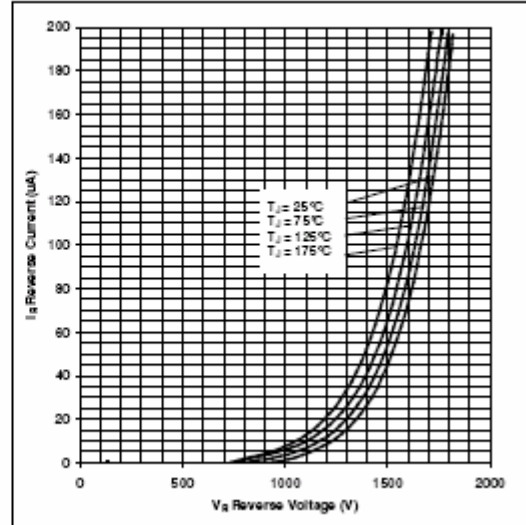
Figure 2. Reverse Characteristics
