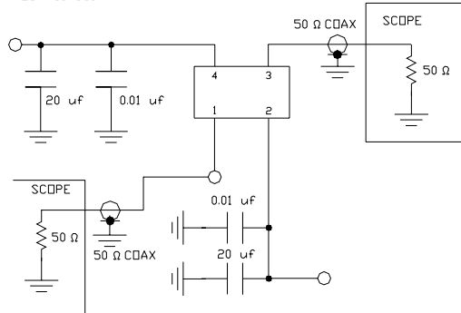
TEST CIRCUIT
