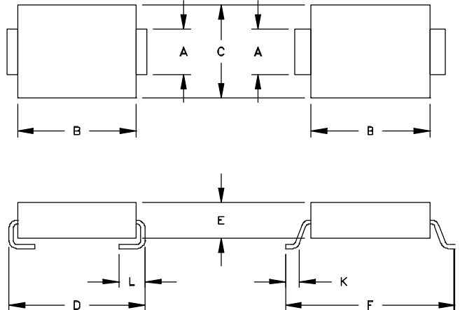
DO-214AB
