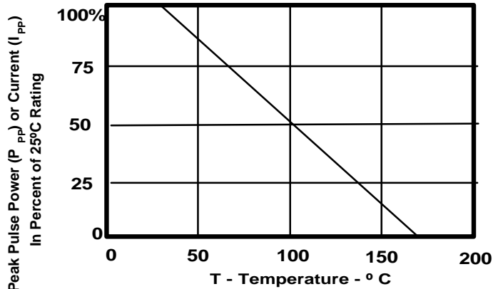
FIGURE 3 Derating Curve
