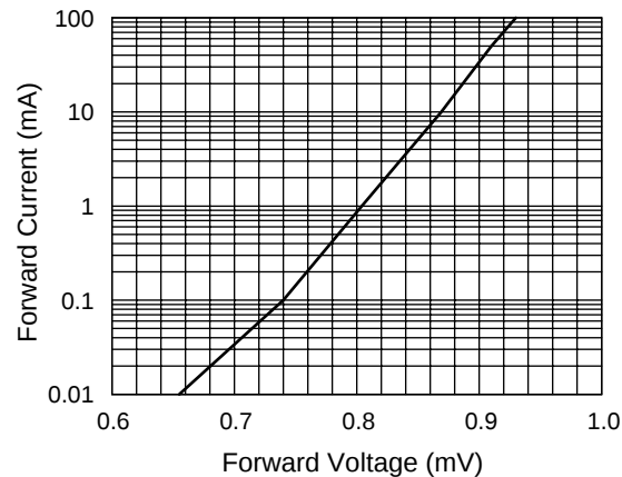
DC Characteristic
