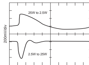
SMTR2805S STEP LOAD RESPONSE
