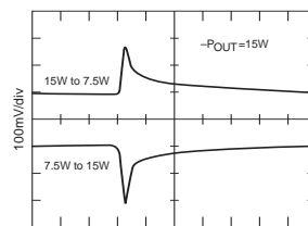
SMTR2815D +VOUT STEP LOAD RESPONSE
