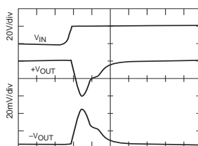
SMTR2815D STEP LINE RESPONSE
