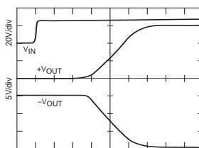
SMTR2815D TURN-ON INTO NO LOAD
