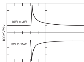
SMTR2815D +VOUT STEP LOAD RESPONSE
