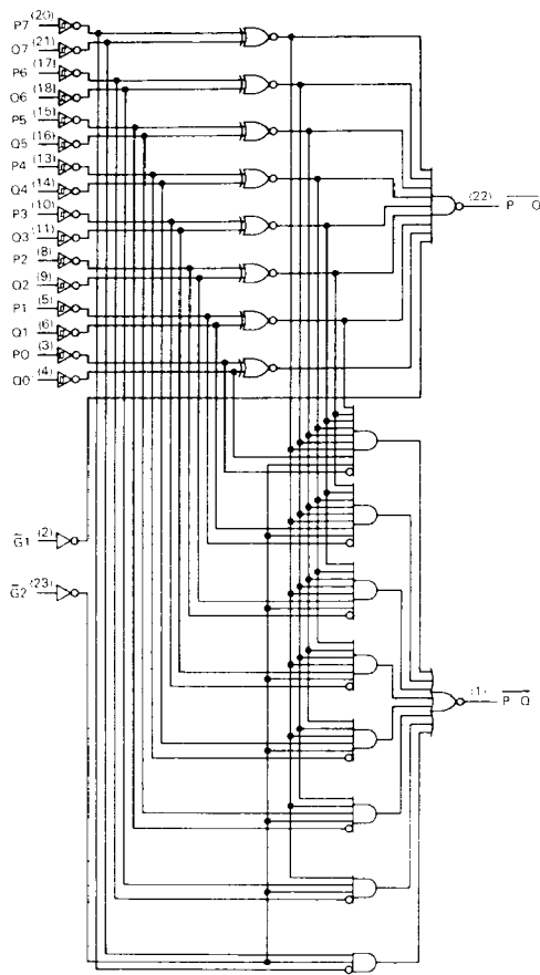
SN54LS/74LS686, LS687
