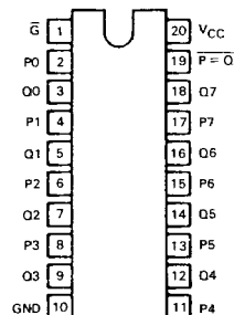
SN54LS/74LS688 SN54LS/74LS689
