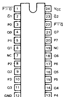
SN54LS/74LS686 SN54LS/74LS687
